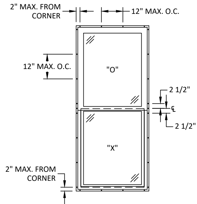
ANCHOR LAYOUT 36" X 84" UNIT
