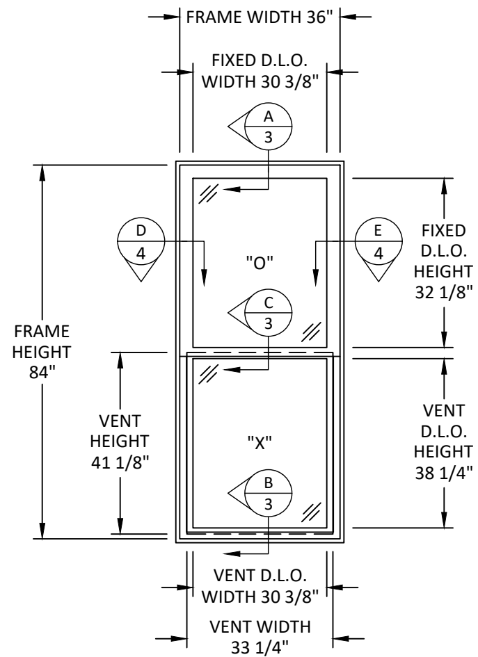
TYPICAL ELEVATION
