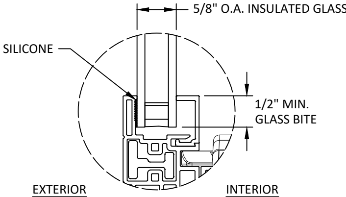
GLAZING DETAIL FIXED LITE
