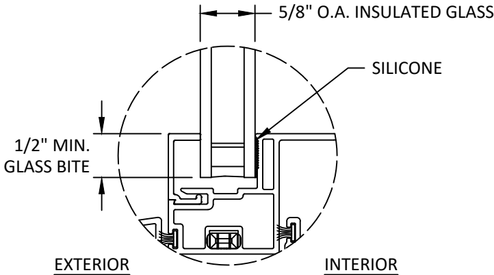
GLAZING DETAIL VENT LITE
