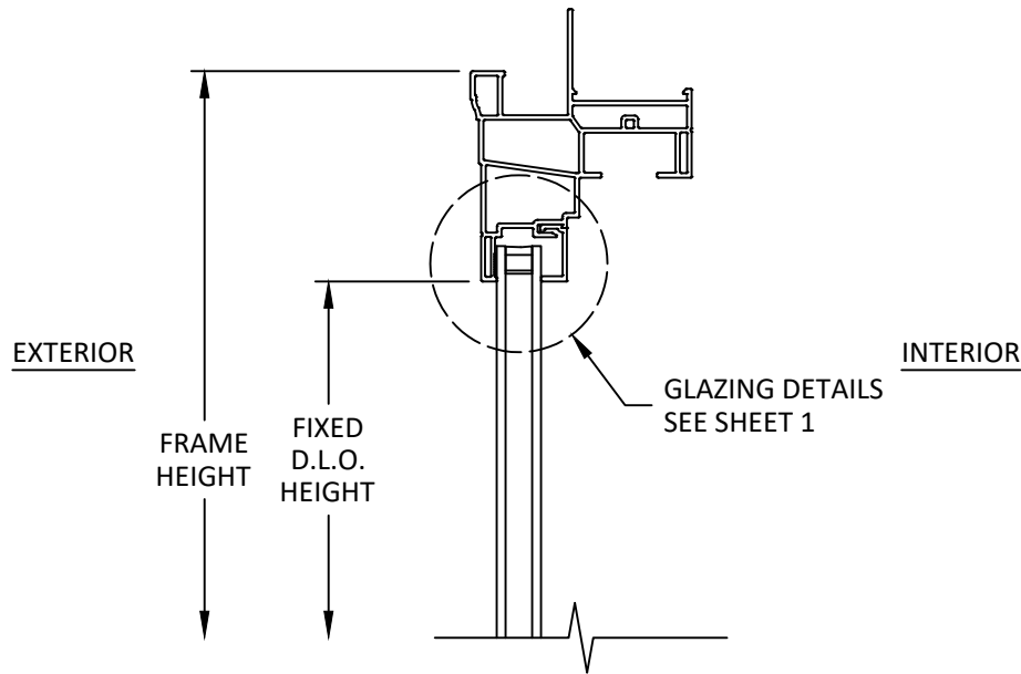
A 3 VERTICAL SECTION HEAD
