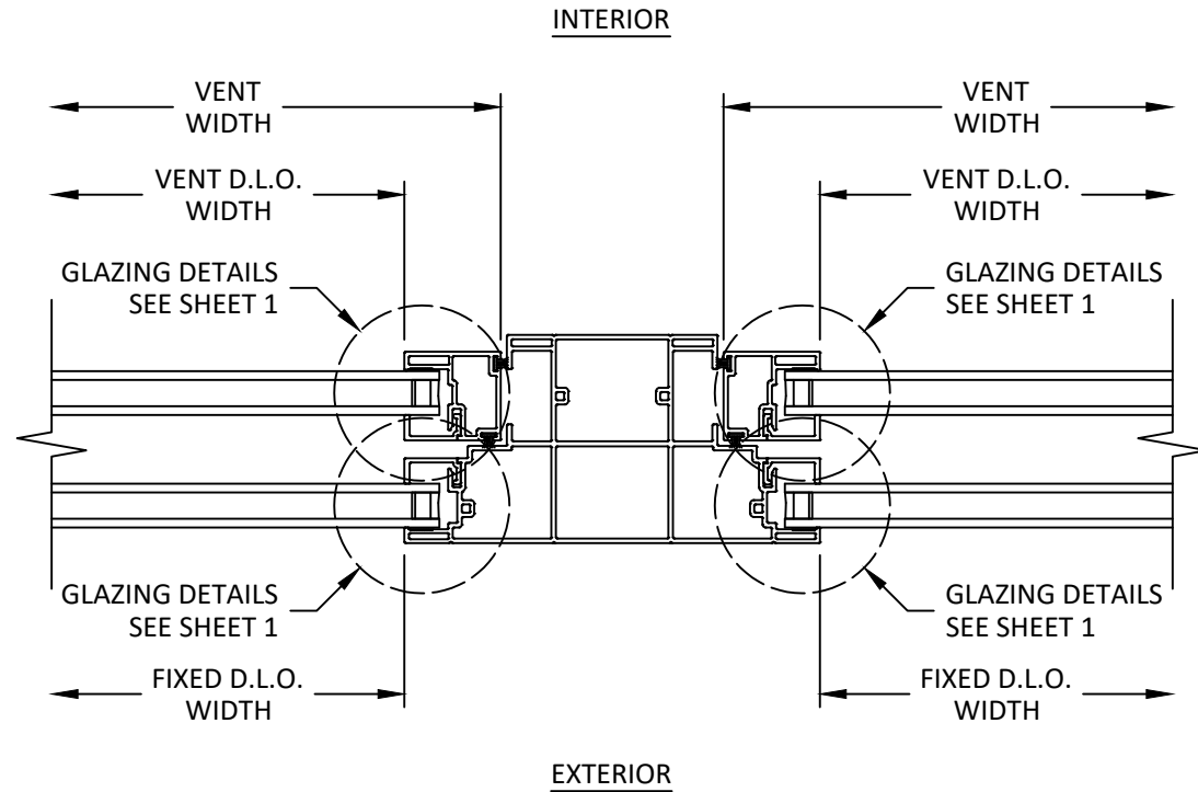
F 4 HORIZONTAL SECTION MULLION
