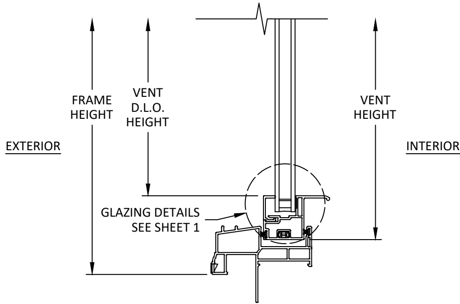
B 3 VERTICAL SECTION SILL
