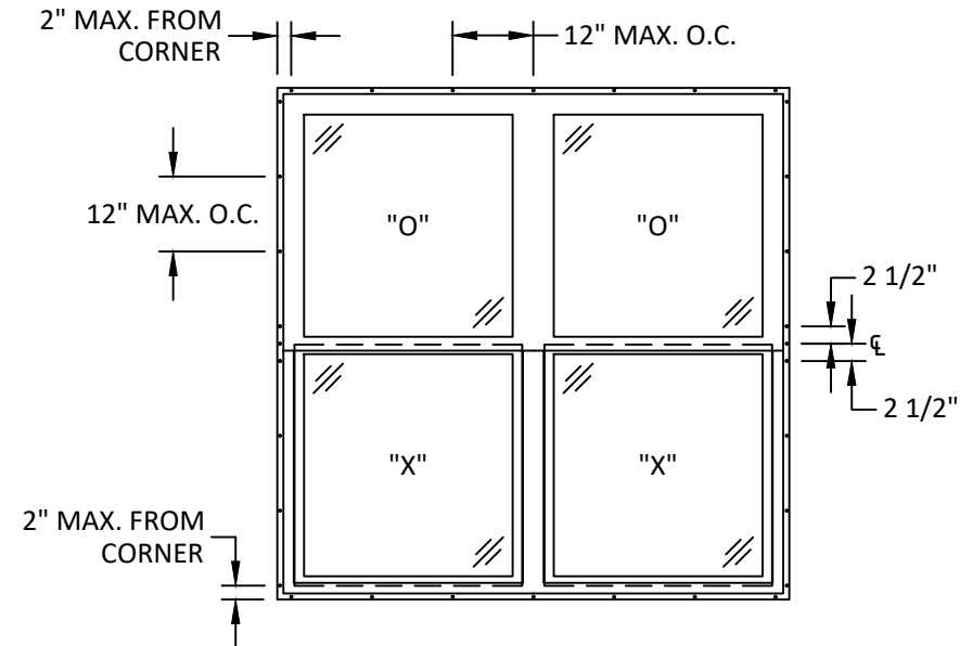
ANCHOR LAYOUT 72" X 72", TWIN UNIT
