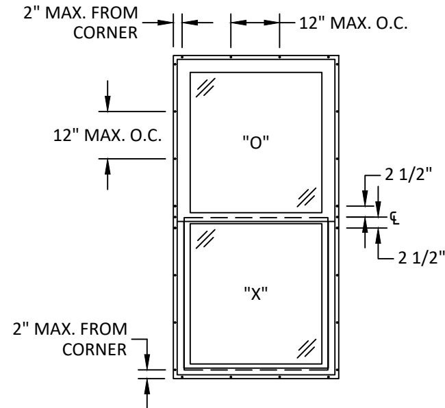
ANCHOR LAYOUT 36" X 72" UNIT
