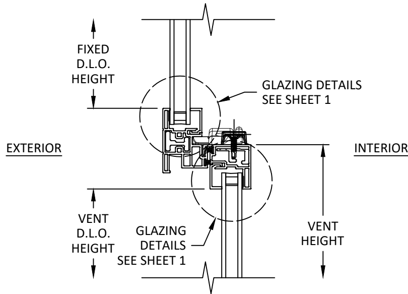
C 3 VERTICAL SECTION MEETING RAIL
