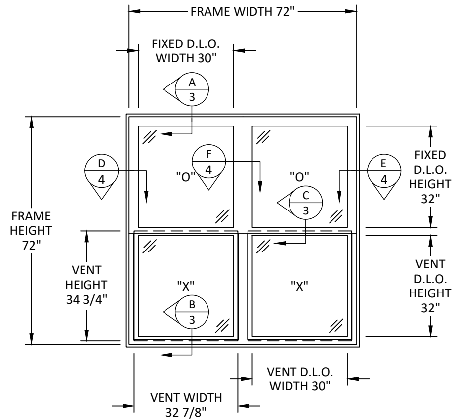
TYPICAL ELEVATION
