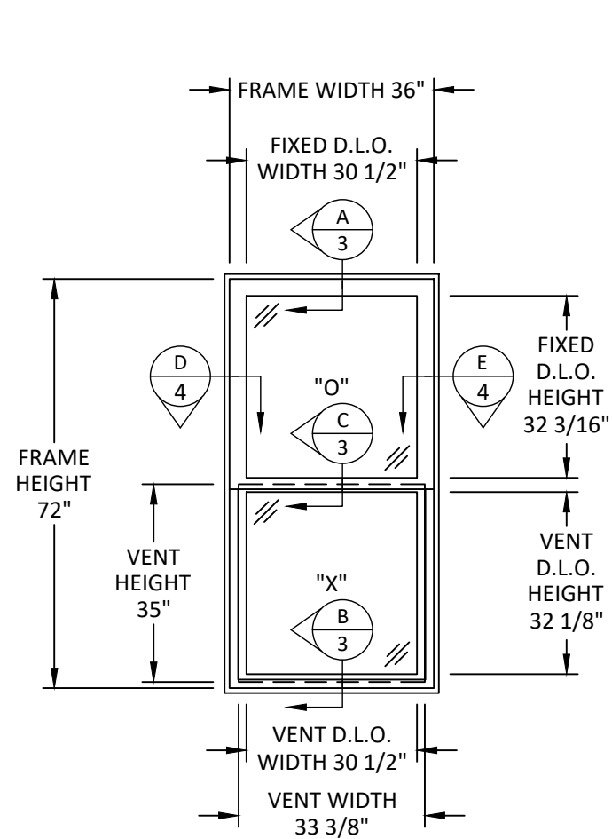
TYPICAL ELEVATION NO KEEPER
